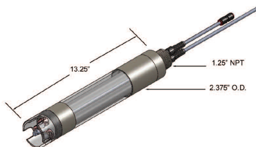
HYDRA® Dimensions
